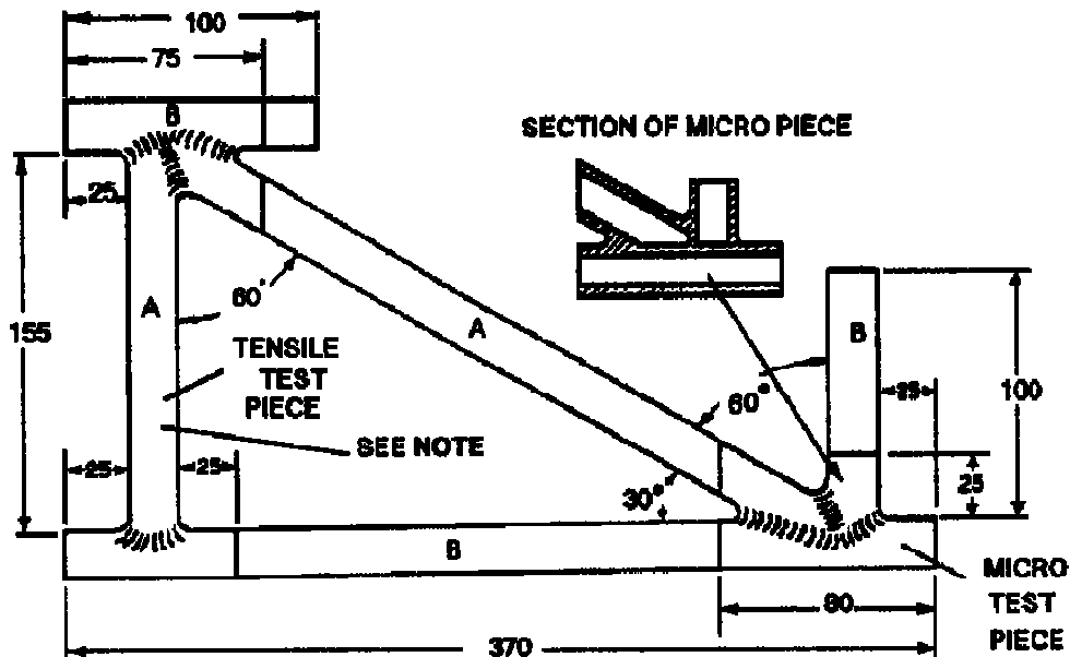
Diagram 4 – Joint No 4 – Tube To Tube Weld
