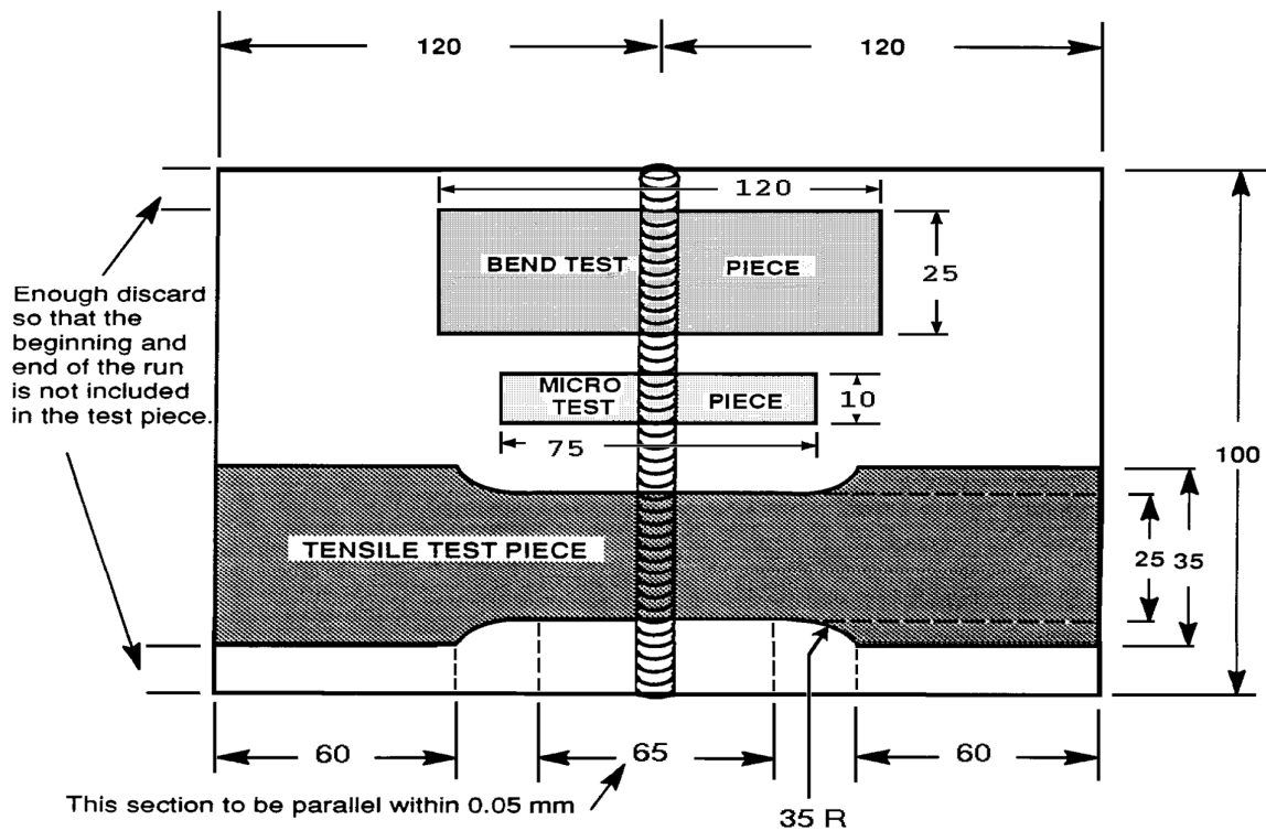
Diagram 1 – Joint No 1 – Sheet to Sheet Butt Weld
