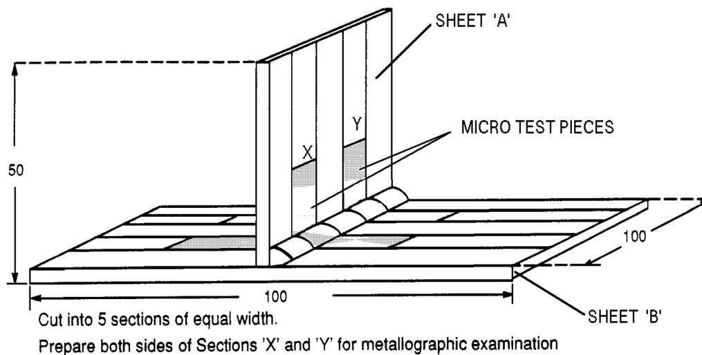
Diagram 3 – Joint No 3 – Sheet to Sheet Fillet Weld
