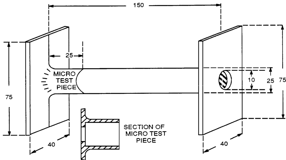
Diagram 2 – Joint No 2 Sheet to Tube Fillet Weld
